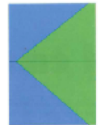
IGDI model
